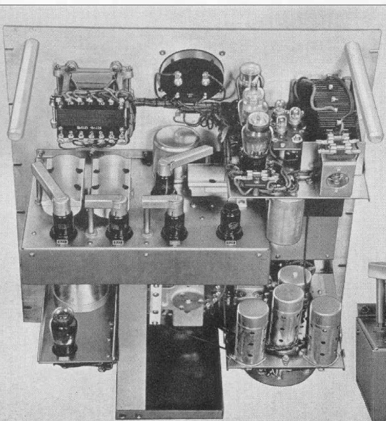
FIGURE 7. Internal view of analyzer showing the mechanical construction. The amplifier (shown also at the right) is of low-impedance aperiodic design; the older type inductive coupling and trimmers are notably absent. The parts are readily accessible. The oscillator is of much more rugged design, which minimizes frequency drifts previously troublesome.
