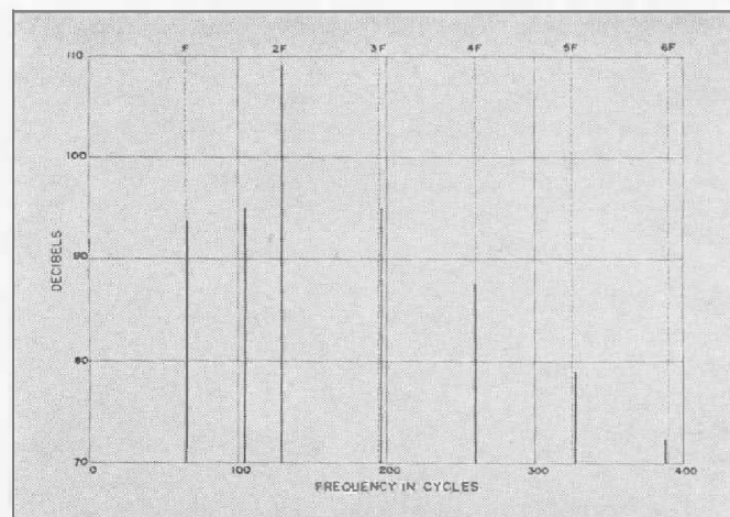
FIGURE 8. Results of measurements made with the TYPE 736-A Wave Analyzer on a phonograph record of airplane noise (courtesy Douglas Aircraft Company).
