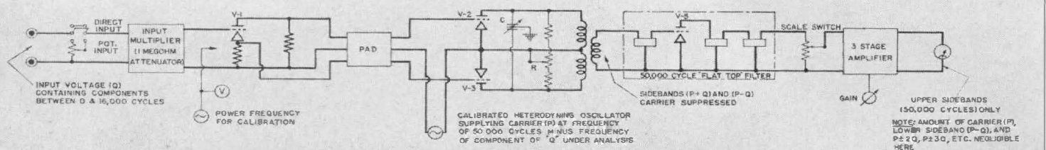
FIGURE 2. Functional schematic diagram showing the principles of operation of the wave analyzer.
