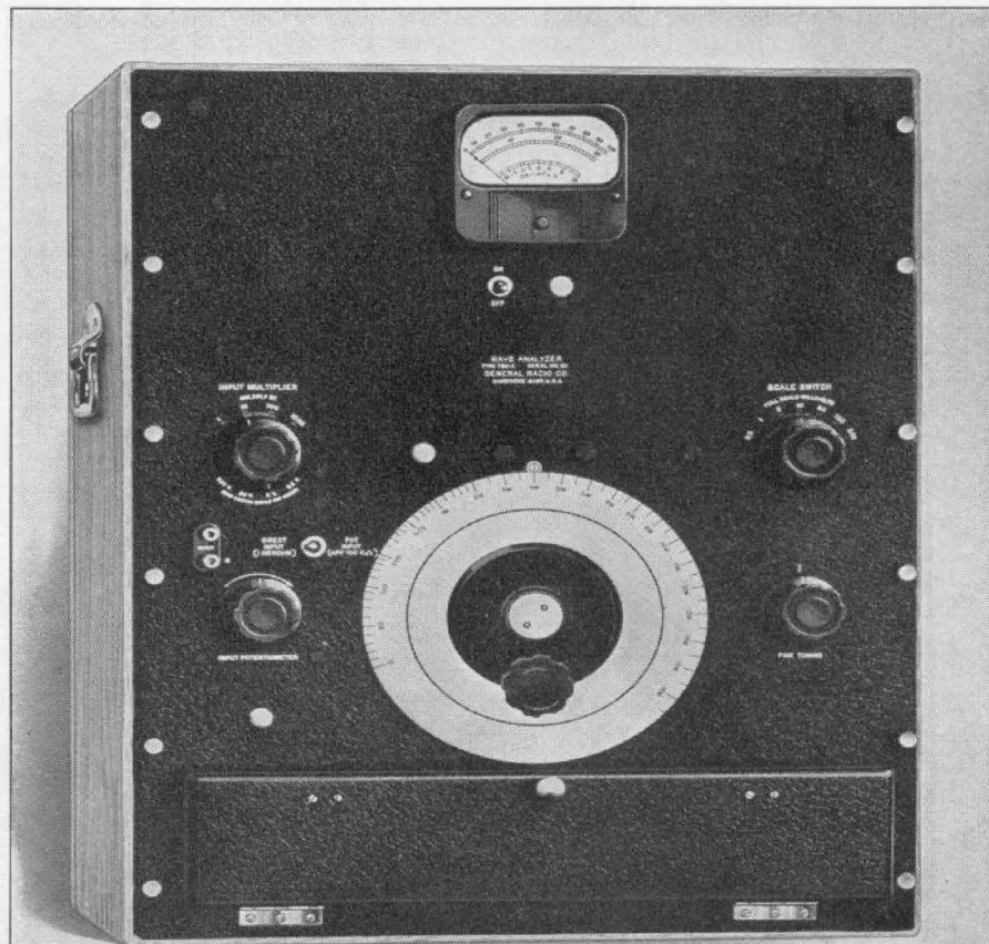
FIGURE 1. Panel view of the TYPE 736-A Wave Analyzer. The panel is standard 19-inch relay-rack width.
