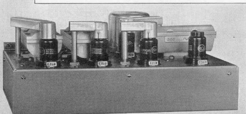
FIGURE 7. Internal view of analyzer showing the mechanical construction. The amplifier (shown also at the right) is of low-impedance aperiodic design; the older type inductive coupling and trimmers are notably absent. The parts are readily accessible. The oscillator is of much more rugged design, which minimizes frequency drifts previously troublesome.
